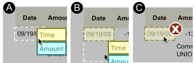
Figure 5: Specifying examples. (A) A menu for specifying examples follows the cursor, jumping to the node under the mouse. (B) After the user clicks “Time”, the system marks the node as a positive example. Positive examples are bordered with the color of the field. Inferred nodes are highlighted but have no border. (C) When the user moves the cursor over a selected node, an X is displayed. The user can click on the X to provide a negative example, turning the border red (Figure 6).
