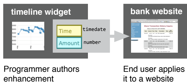
Figure 1: reform divides web enhancement into roles of authoring, for programmers, and attaching, for end users.
