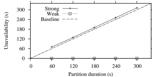
Figure 2: Varying partition durations with no concurrent operations. Baseline represents the minimal unavailability expected for strong operations, which is equal to the partition duration.
