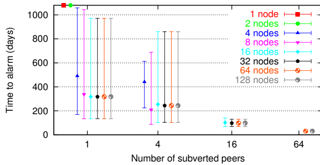
Fig. 9. Time from start of nuisance attack to first alarm at any peer ( y axis) versus the number of peers subverted ( x axis), for varying adversary resource sizes. Some attacks with few subverted peers do not cause alarms in our timescale.
