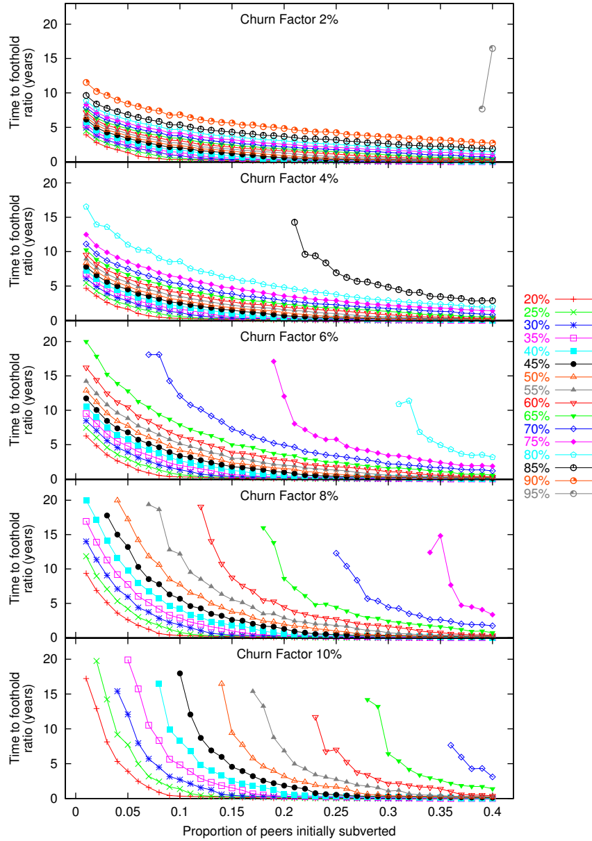
Fig. 3. Minimum time for the stealth adversary to achieve various foothold ratios, starting with various proportions of initially subverted peers. We show graphs for churn factors 2, 4, 6, 8, and 10%.
