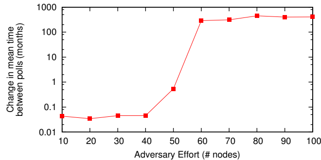
Fig. 10. Effect of the attrition adversary in increasing mean time between polls as a function of his effort. The y axis is in logarithmic scale.
