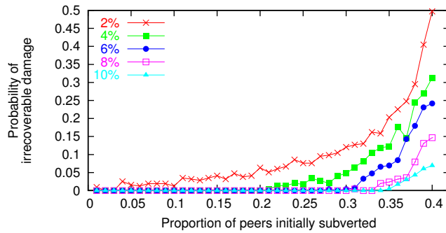
Fig. 8. Probability that the adversary causes irrecoverable damage. Each curve corresponds to a different churn factor.
