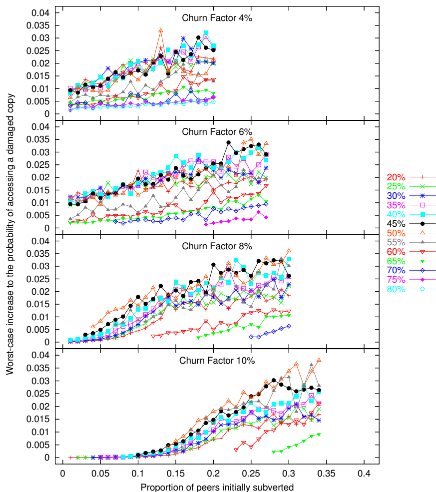
Fig. 6. Worst-case increase in the probability of accessing a bad replica due to the attack, as a function of initial subversion. Each curve corresponds to runs with a different foothold ratio at the start of the attack phase. We only show values for subversions at which the adversary did not cause irrecoverable damage. We show graphs for churn factors of 4, 6, 8 and 10%.
