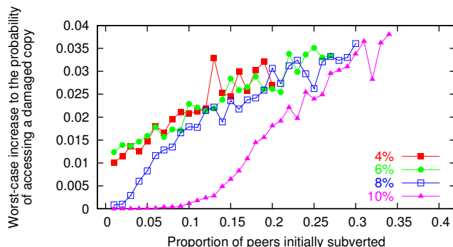
Fig. 7. Worst-case increase in the probability of accessing a bad replica due to the attack, as a function of initial peer subversion. Each curve corresponds to runs with different churn factors. We only show values for subversions at which the adversary did not cause irrecoverable damage, for each churn.
