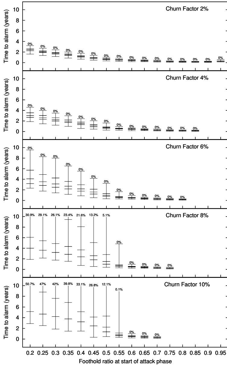
Fig. 4. The time from the start of the attack phase (in the stealth strategy) to the time of detection, for different starting reference list foothold ratios. Ticks split the value distributions into quartiles. Percentages above the distributions indicate runs that did not generate an alarm. We show graphs for churn factors 2, 4, 6, 8, and 10%.
