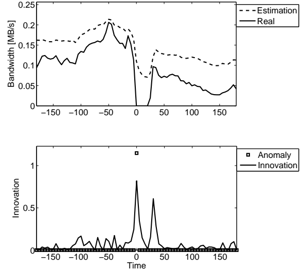
Figure 6: Example 2 of the Innovation of an OD pair.
