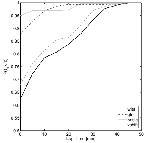
Figure 7: CDF of detection lag for Abilene traces.
