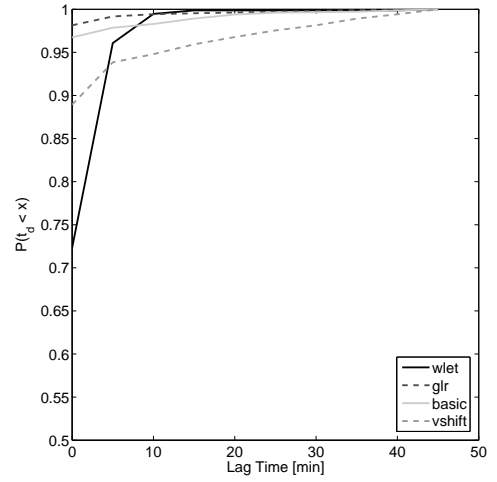
Figure 8: CDF of detection lag for synthetic anomalies.
