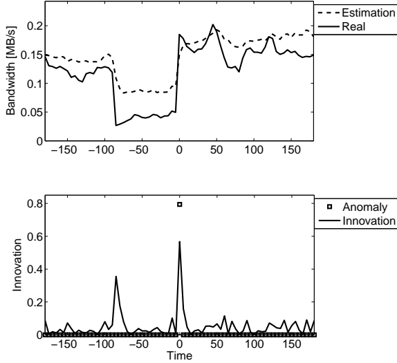
Figure 5: Example 1 of the Innovation of an OD pair.
