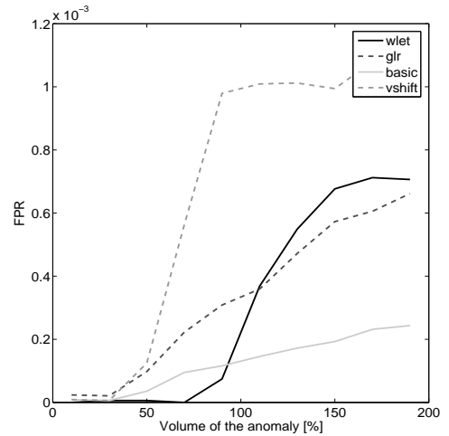
Figure 10: FPR as a function of the anomaly size.
