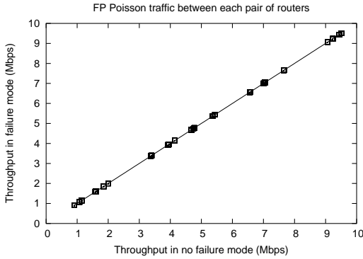
Fig. 14. Throughput for FP traffic: failure mode versus no failure mode.
