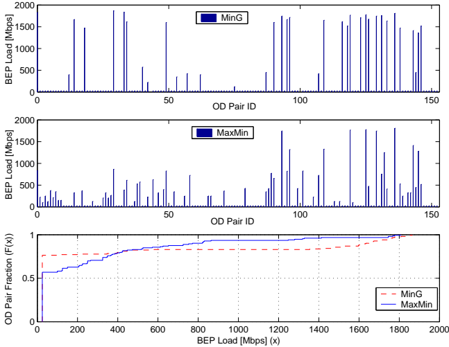
Fig. 12. BEP load distribution among the logical connections for the two fairness policies introduced with a Z_{min} = 25 Mbps.
