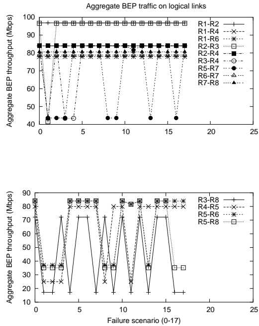
Fig. 21. Average throughput for BEP traffic for each failure scenario.
