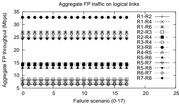
Fig. 20. Average throughput for FP traffic for each failure scenario.
