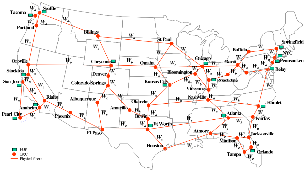
Fig. 10. Sprint WDM Topology: 36 OXC with 55 WDM fibers. Heterogeneous backbone: W_a represents an OC192 system equipped with 40 channels at 10 Gbps, W_b represents an OC48 system with 40 channels at 2.44 Gbps and W_c an OC12 system with 40 channels at 622 Mbps.
