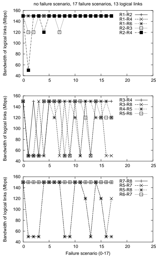
Fig. 13. Bandwidth of each logical link (13 in total) in the normal operation state (failure id 0) and for any physical link failures (failure id from 1 to 17).
