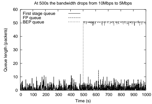
Fig. 4. Occupancy of the three buffers of the scheduler
