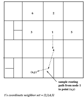
Fig. 6. Example 2-d space
