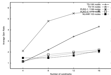
Fig. 3. Effect of number of landmarks (#levels = 1)
