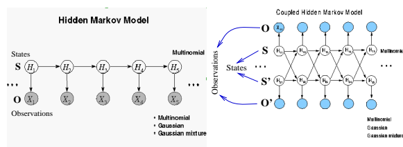
Figure 4: Graphical representation of HMM and CHMM rolled-out in time
