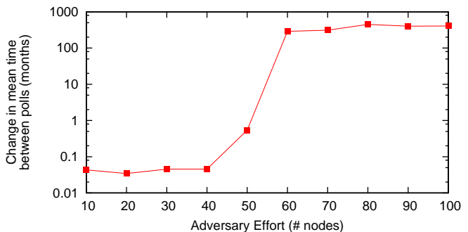
Fig. 2. Change in the mean time between LOCKSS polls, as a function of the computational power of the attrition adversary. The y axis is in logarithmic scale. There are 1000 peers in the system.
